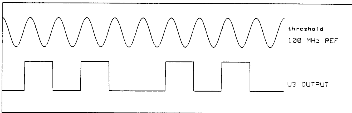
Figure A39-1. A39 PLL3 Frequency Multiplier Waveforms.
