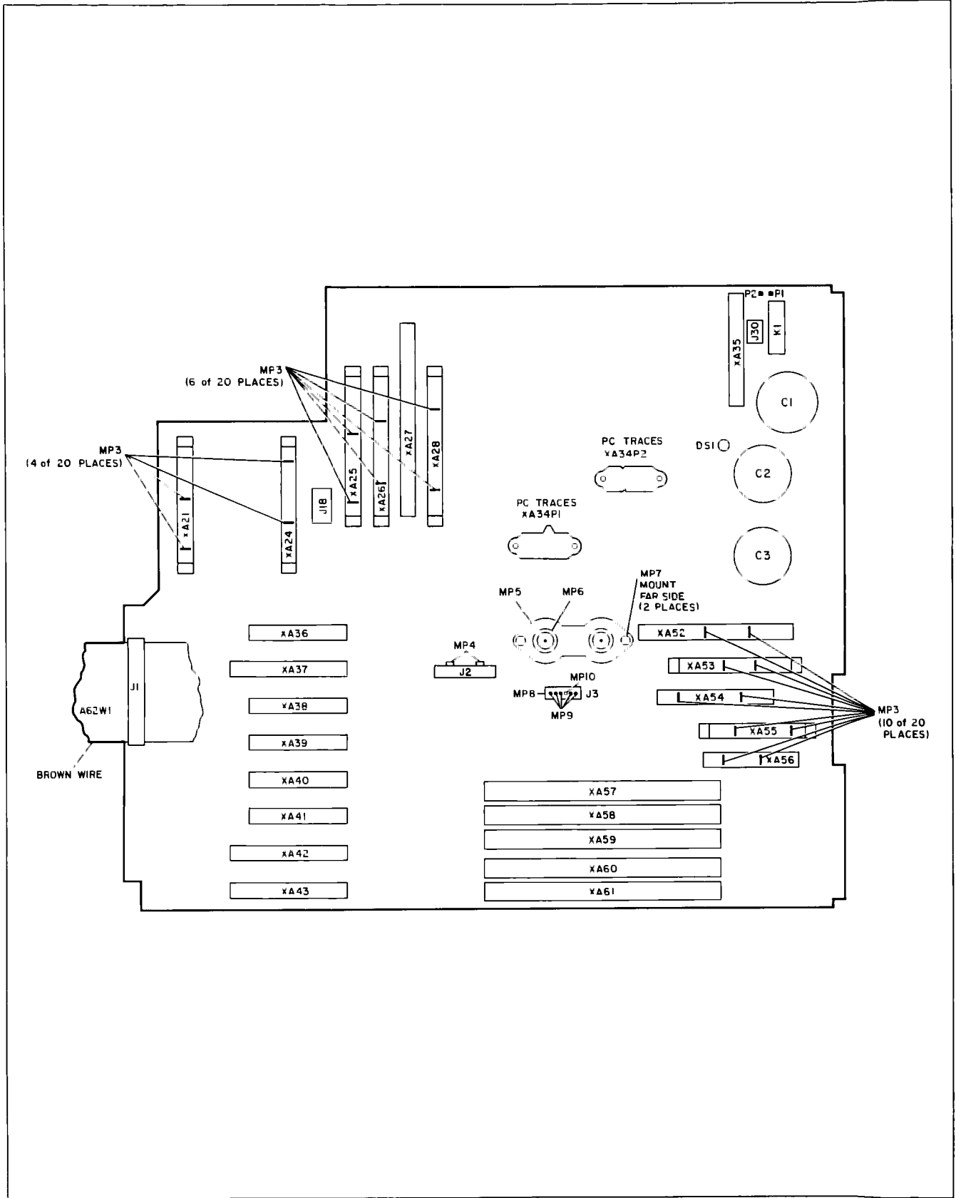
Figure A62-2. A62 Motherboard Component Location Diagram (1 of 2)
